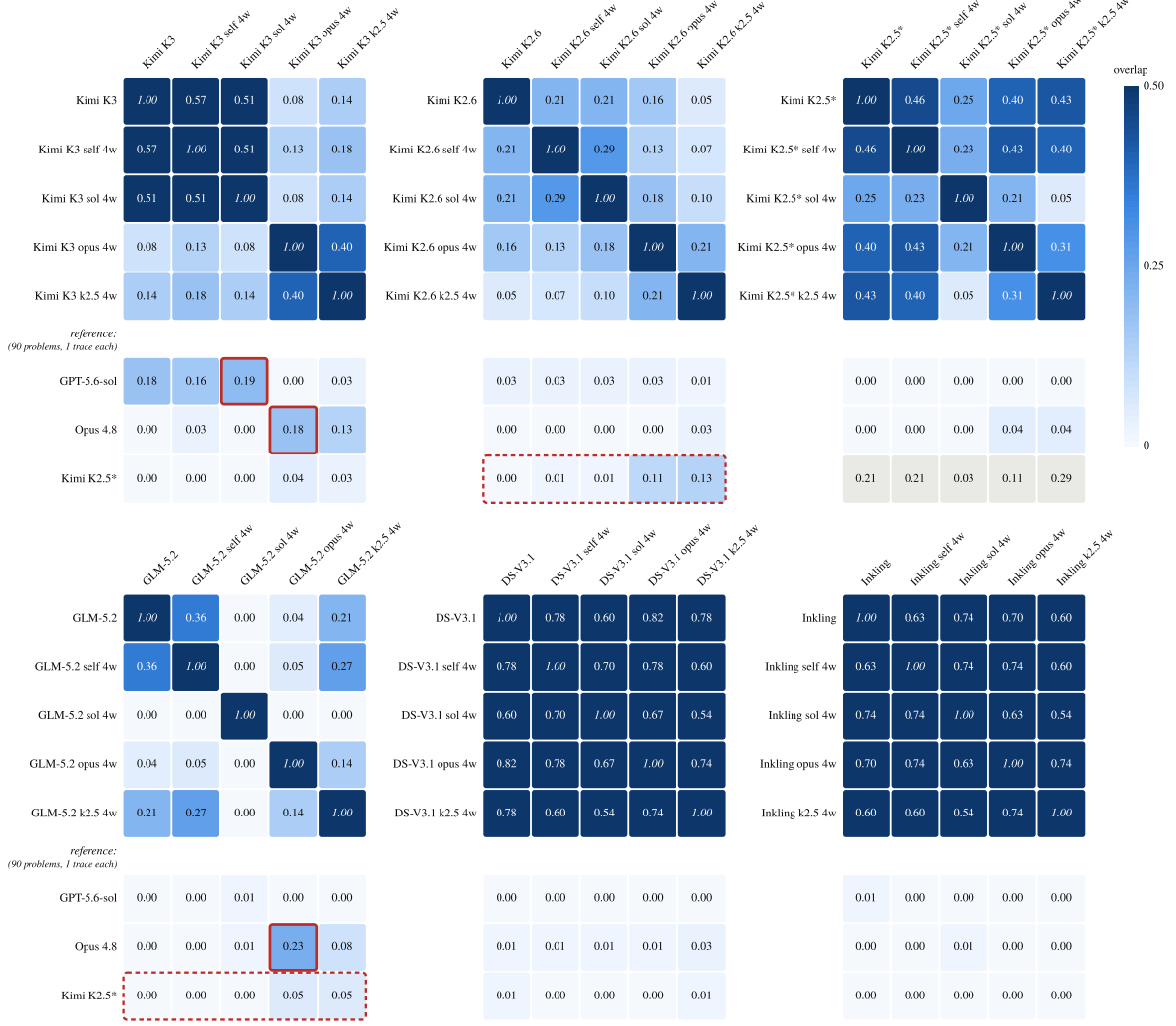
Figure 29: Distinctive n-gram overlap under prefills. Each cell reports the Jaccard overlap of the two rows’ most characteristic n -grams, scored against the pooled unpre-filled controls as described in Appendix B.4.3. Darker hue indicates more shared n -grams and the diagonals are one by definition. The square blocks show the same five conditions as Figure 27. The reference cells are near or at zero everywhere except the Kimi-K3 vs Sol cells, the three cells outlined in red, and a few Kimi-K2.5-prefill cells. Sol-prefilled Kimi-K3 shares characteristic n -grams with the Sol reference (0.19, from 0.18 without any prefill). Opus-prefilled Kimi-K3 and GLM-5.2 share n -grams with the Opus 4.8 reference (0.18 and 0.23). The control-versus-self cells compare the self-prefilled traces against the exact control trace whose opening was pre-filled, one per problem. The reference cells of the self column match the unpre-filled ones to within 0.03. In the Kimi-K2.5 reference row, the gray cells compare Kimi-K2.5 with its own teacher traces, and Kimi-K2.6 shows a small overlap with the teacher chiefly under the Kimi-K2.5 prefill (0.13, dotted red row) and to a lesser degree under the Opus prefill (0.11). Note that Kimi-K2.5 is truncated at its 8,192-token serving cap in all rows due to prefill-API limitations.
